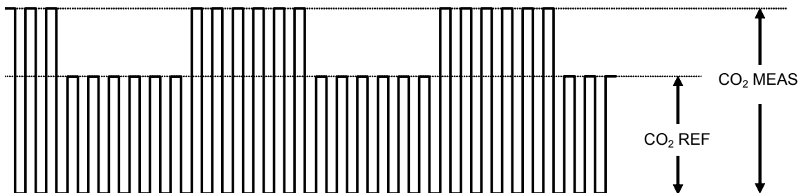
Figure 7-6: Chopped IR Signal
